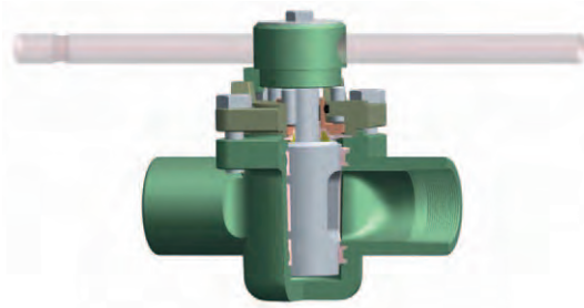
FIG. P250SC 316/316
