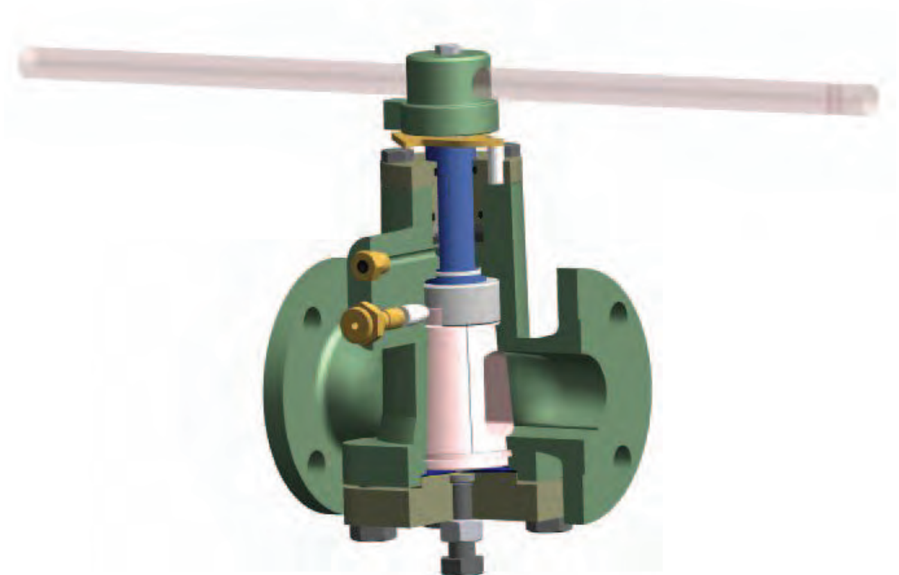
FIG. P260L WCB/WCB PRESSURE BALANCED PLUG VALVES
