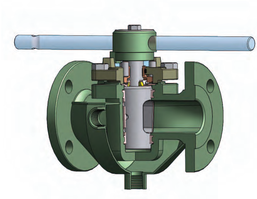
FIG. P250PJ 316/316/304 TEFLON SLEEVED JACKETED PLUG VALVES
