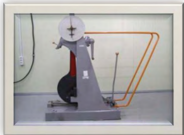
IMPACT TESTER
